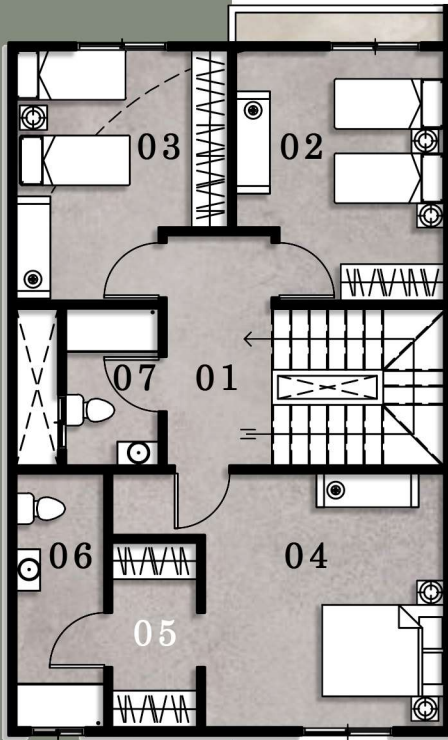
First Floor Area: 82m 2
