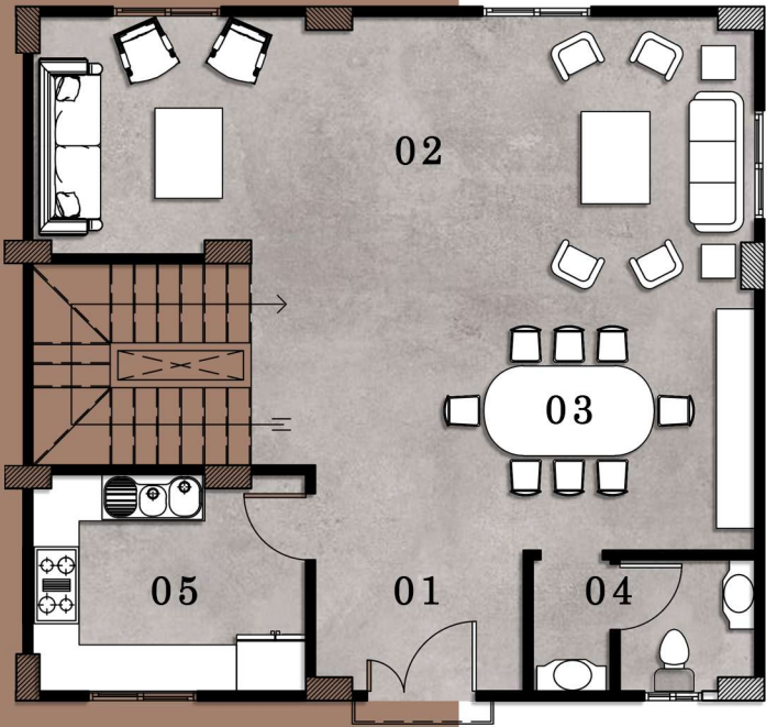
Basement Floor Area: 86m2
