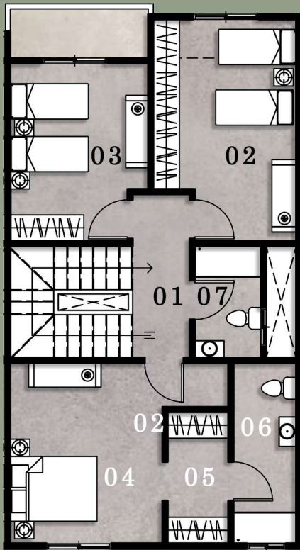
First Floor Area: 81m 2
