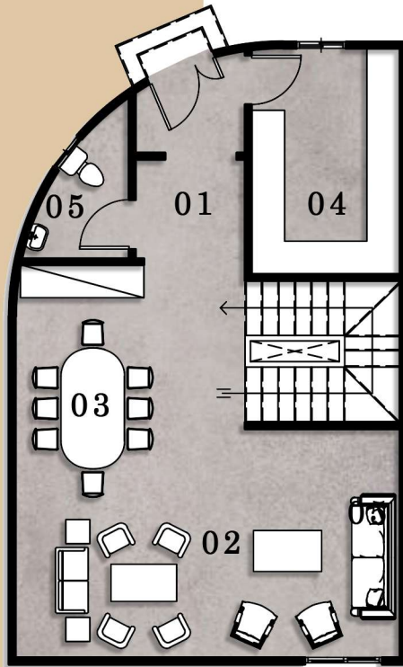
Ground Floor Area: 77m 2
